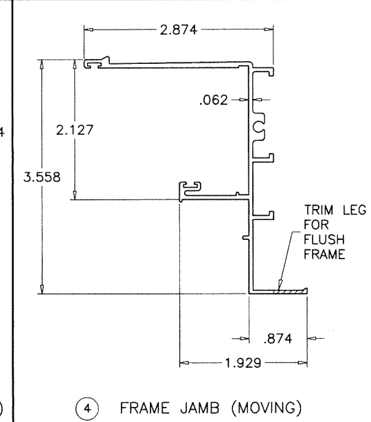
③ FRAME JAMB (MOVING/FIXED)
